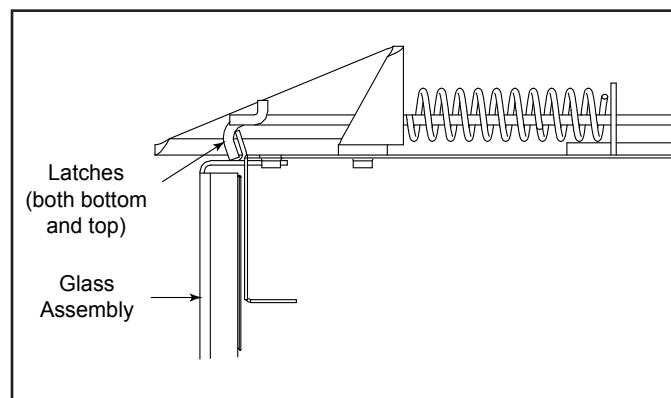
Figure 4.1 Glass Assembly
