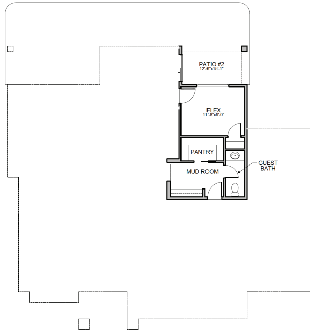
1C. FLEX ROOM w/ PATIO #2
